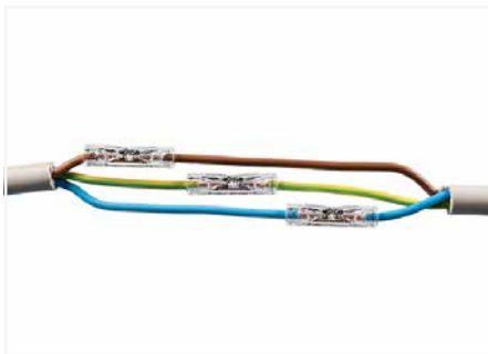
Strip 10 mm conductor per specification and insert connector (example shows staggered connectors).
